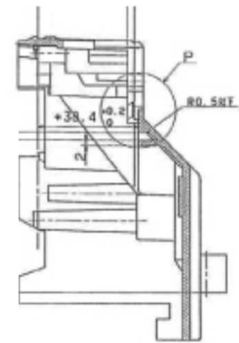
SEC I-I
